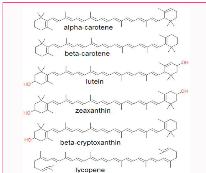
Figure 18: Carotenoids Structure.
