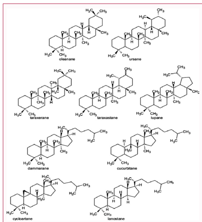
Figure 17: Chemical structures of the main subclasses of triterpenes [38].
