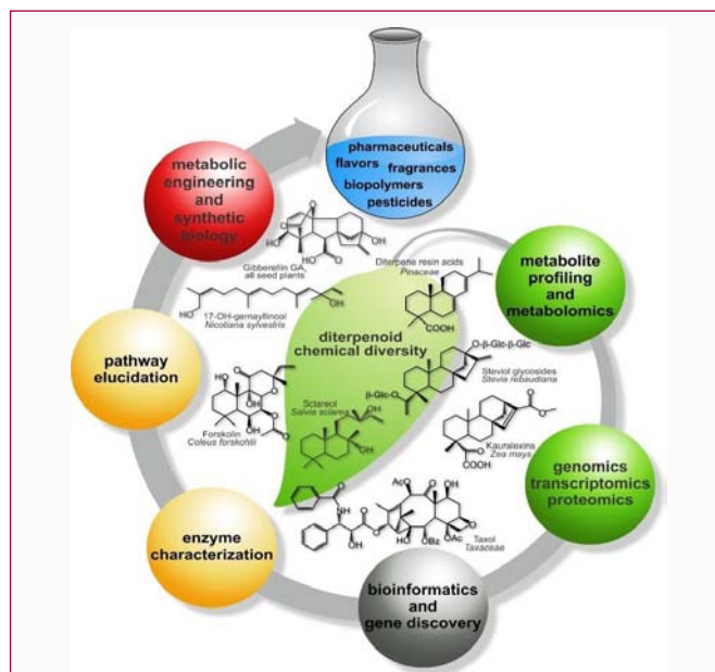
Figure 4: Functional genomics enable efficient discovery of terpene metabolic pathways [5]. So as to explore and eventually outfit the huge chemical collection of plant terpenoid metabolism, a center quality of our lab is the effective distinguishing proof of terpeneid-metabolic qualities, catalysts and pathways by consolidating genomics-empowered quality revelation utilizing in-house protein databases, quick compound biochemical portrayal through microbial and plant co-articulation measures, and all over again ID of novel metabolites utilizing mass spectrometry and NMR approaches. Utilizing these instruments, we have recognized more than 50 practically particular TPS and P450 proteins in over twelve plant species with pertinence for nourishment, bioenergy and prescription. We coordinate these biochemical bits of knowledge with in planta terpenoid profiling by means of GC- and LC-MS examinations, hereditary quality capacity contemplates utilizing CRISPR/Cas9-empowered pathway adjustment, just as plant-condition cooperation thinks about utilizing in vitro and in vivo plant-pathogen and plant-microbiome investigations to research the bioactivity of terpenoid metabolites and assess their potential for agrarian and other biotechnology applications.
