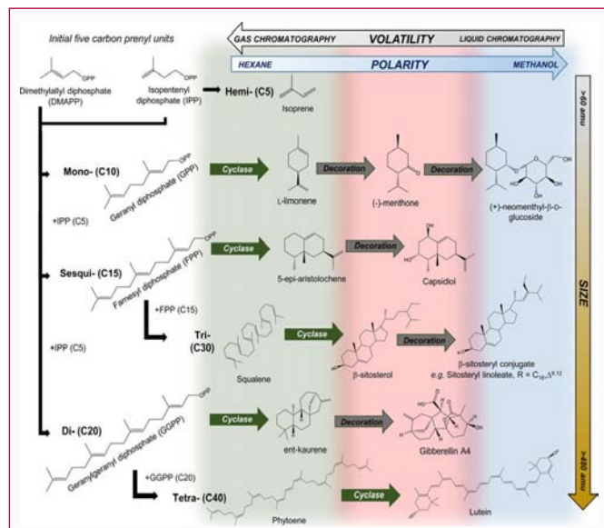
Figure 3: A schematic depiction of terpene metabolism emphasizing the biosynthesis of the different classes of compounds and their physical properties (volatility and polarity) [2]. DMAPP and IPP are the fundamental structure squares used to create the allylic diphosphate forerunners explicit to every terpene class: GPP for monoterpenes; FPP for sesquiterpenes and triterpenes; and GGPP for diterpenes and tetraterpenes. Ionization of the phosphorylated antecedents yields straight hydrocarbon frames, while the coupled ionization/cyclization responses catalyzed by synthases/cyclases yield an inconceivably rich cluster of cyclized hydrocarbons. These straight and cyclized hydrocarbon frameworks are commonly nonpolar or mono-hydroxylated, and their unpredictability is associated with their sub-atomic mass. The littler exacerbate, the more unstable they will be. Be that as it may, all these terpene platforms are likewise subject to extra layers of alteration including hydroxylations, glycosylations, acylations, and aroylations, which adjust the physical size and nature of the terpene particle, and can expand their extremity. This figure is additionally shading coded in reference to the conventions talked about here which may be the most productive for extraction, quantitation and auxiliary distinguishing proof of the individual terpene particles. Convention 1 is intended for to a great extent nonpolar compounds and is featured in green; Protocol 2 is for those atoms having an increasingly polar nature (red); and those terpenes having the best extremity are most likely best extricated, evaluated and qualified by Protocol 3 (blue).
