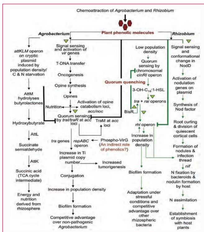
Figure 19: The use of phenolics by Agrobacterium and Rhizobium for survival and infection of the host plant [49]. Black arrows show how Agrobacterium utilizes phenolics to start an intricate procedure of pathogenesis, finishing with opine blend. Notwithstanding their dietary benefit, opiines help Agrobacterium 's opposition with nonpathogenic microbes, for example, A. radiobacter , by expanding its populace thickness and biofilm arrangement through majority detecting. Agrobacterium likewise utilizes the attKLM operon to manage its populace thickness amid times of dietary starvation and to integrate elective wellsprings of supplements and vitality by debasing g-butyrolactones created by other rhizospheric microorganisms. Green bolts demonstrate the utilization of phenolics by Rhizobium leguminosarum viciae for the enlistment of gesture qualities pursued by the procedure of advantageous interaction. Under pressure conditions, phenolics likewise manage the expansion in populace thickness, biofilm development and compelling nodulation by subduing the majority detecting rhi operon. An expansion in populace thickness because of majority detecting gives an aggressive edge to rhizobia over other rhizospheric microorganisms. Striking lines demonstrate the majority extinguishing components, though triangles speak to the means of actuation. TCA: Tricarboxylic Corrosive.
