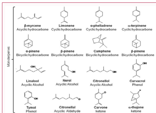
Figure 5: Examples of some mono-terpenes compounds found in essential oils of plants [8].
