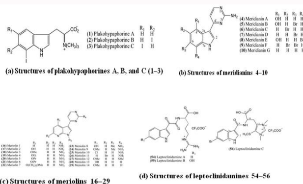
Figure 49: Halogenated Indole Alkaloids from Marine Invertebrates [134].
