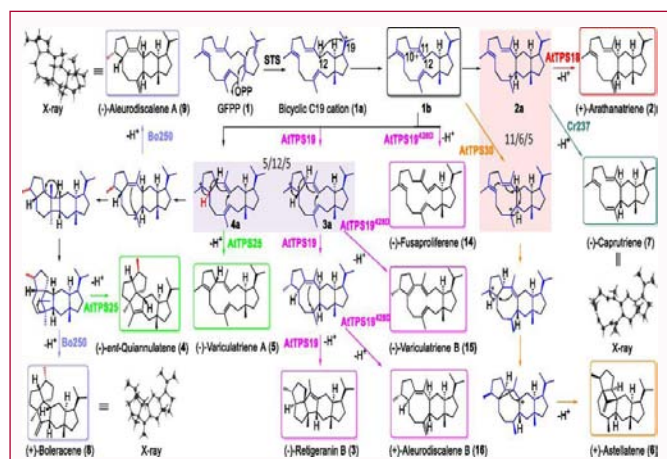
Figure 16: Proposed cyclization paths toward the formation of fungal-type sesterterpenes 2–9 and 14–16 by plant STSs [32]. The universal sesterterpene precursor GFPP is cyclized to form the unified bicyclic C12 cation 1b (black box) following protonation in the active sites of plant STSs and mutated AtTPS19 (AtTPS19428D). Cation 1b diverges to 5/12/5 and 11/6/5 tricyclic carbocations en route to the formation of (+)-arathanatriene (2), (–)-retigeranin B (3), (–)-ent-quiannulatenene (4), (–)-variculatriene A (5), (+)-astellatene (6), (–)-caprutriene (7), (+)-boleracene (8), (–)-aleurodiscalene A (9), (–)-fusaproliferene (14), (–)-variculatriene B (15), and (+)-aleurodiscalene B (16). Compounds isolated and characterized are highlighted in colored boxes. Different colors indicate different cyclization paths. Crystal structures 7–9 are presented with displacement ellipsoids shown at 50% probability.
