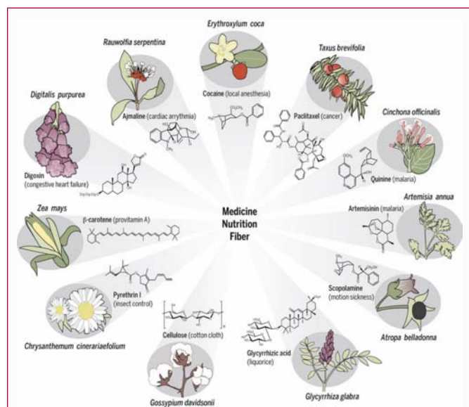
Figure 1: Selected plants and their uses [1]. Since the beginning, plants have filled in as wellsprings of a plenty of chemicals that give mankind prescription, fiber, and nourishment. The chemical assorted variety of plants is tremendous. Plants developed the biosynthesis of a cornucopia of novel chemicals to endure and convey in a complex natural condition. Albeit some plant chemicals are sharp or harsh tasting (glucosinolates and pyrrolizidine alkaloids) to stop herbivory, others, for example, anthocyanins and carotenoids are brilliantly hued blossom shades that draw in pollinators. Chemicals that are cytotoxic or generally physiologically dynamic in warm blooded creatures are utilized, for instance, as agony executioners, chemotherapeutics, and different medications. These plant chemicals are made through species-explicit, specific biochemical pathways that adjust metabolites of essential metabolism. A plenty of new chemicals and metabolic pathways are likely covered up in plant genomes anticipating revelation. In spite of the fact that structures for 200,000 natural products are known, just 15% of the evaluated 350,000 plant species have been examined for their chemical constituents.
