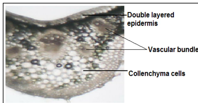
Fig 2: T/S of midrib of P. hirsuta leaf
