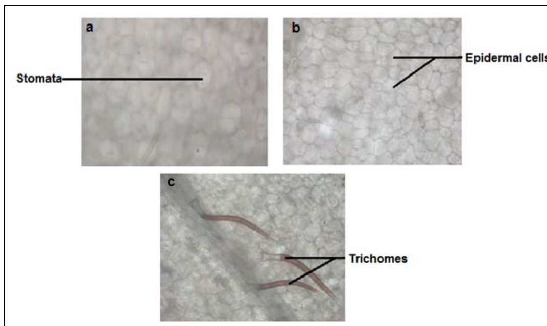
Fig 3: Leaf surface features of P. hirsute
