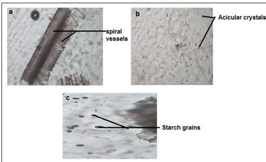
Fig 4: Powder microscopy of P. hirsuta leaves
