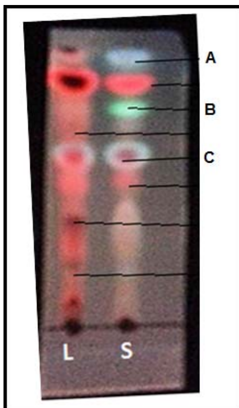
Fig 5: TLC chromatogram of the leaf and stem of P. hirsuta visualised under UV (365nm) L: leaf extract, S: stem extract
